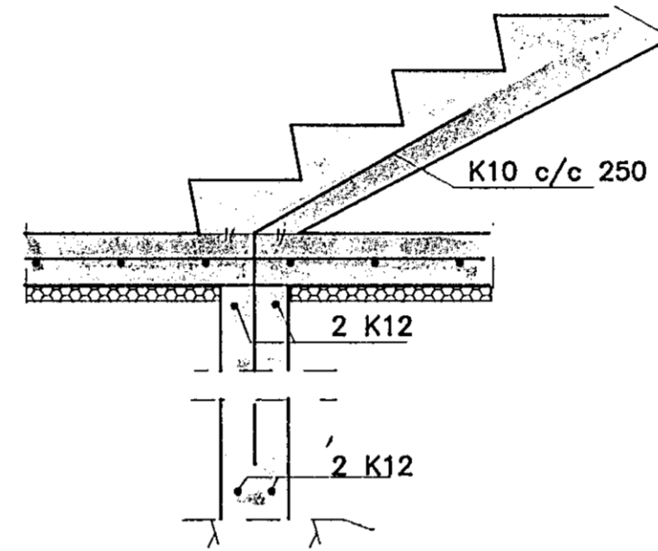
SNID C-C 1:20
