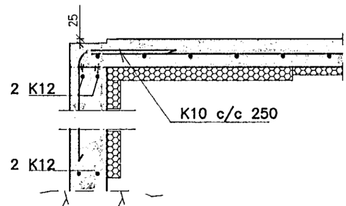
SNID E-E 1:20
