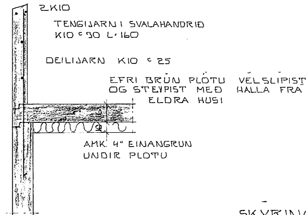
SNID C-C 1:20
