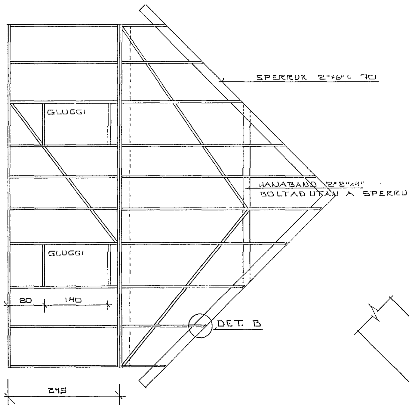
VEGGGRIND GAFL 1:50
