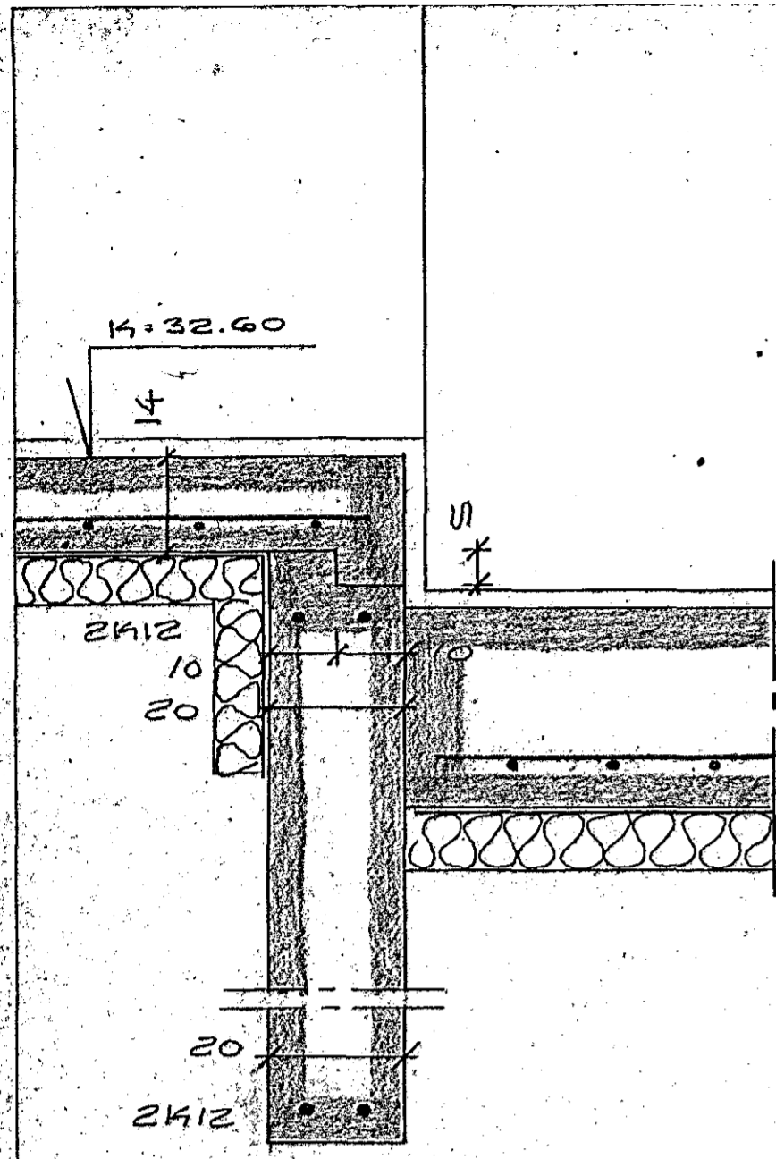
SNID H-H, M=1:10
