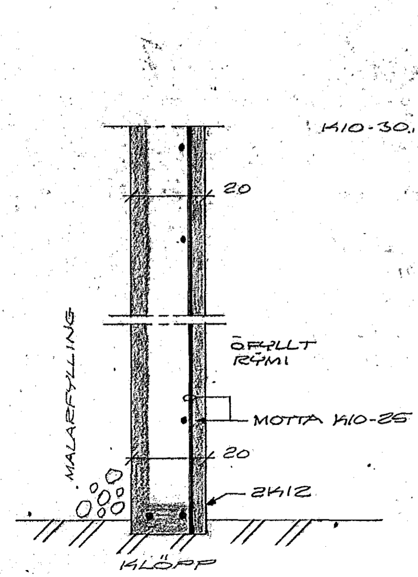
SNID A, M=1:10
