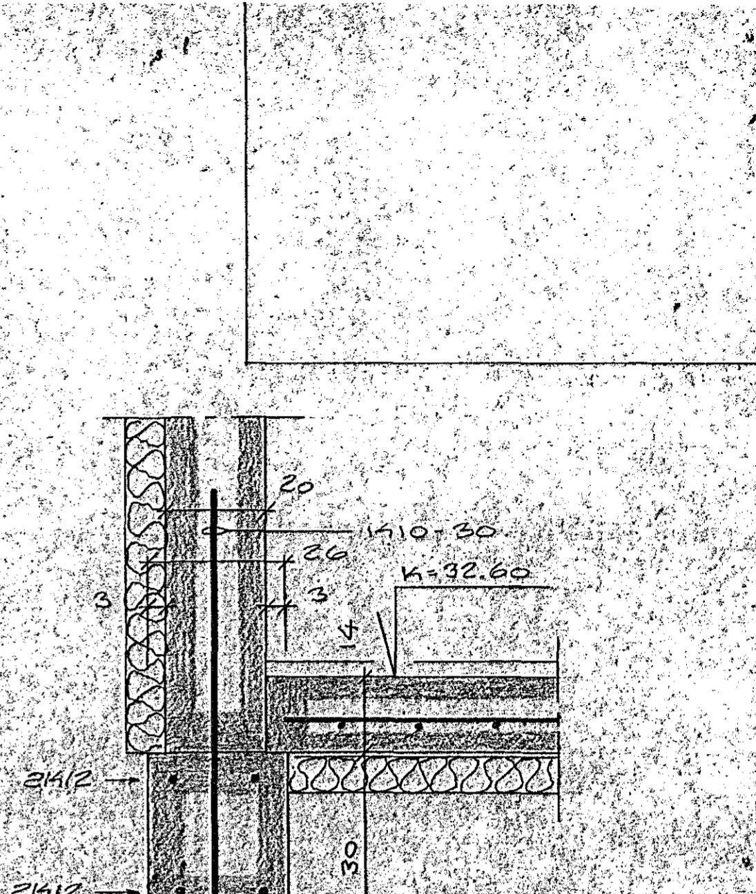
SNID E-E, M=1:10
