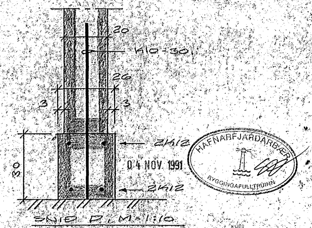
SNID D, M=1:10
