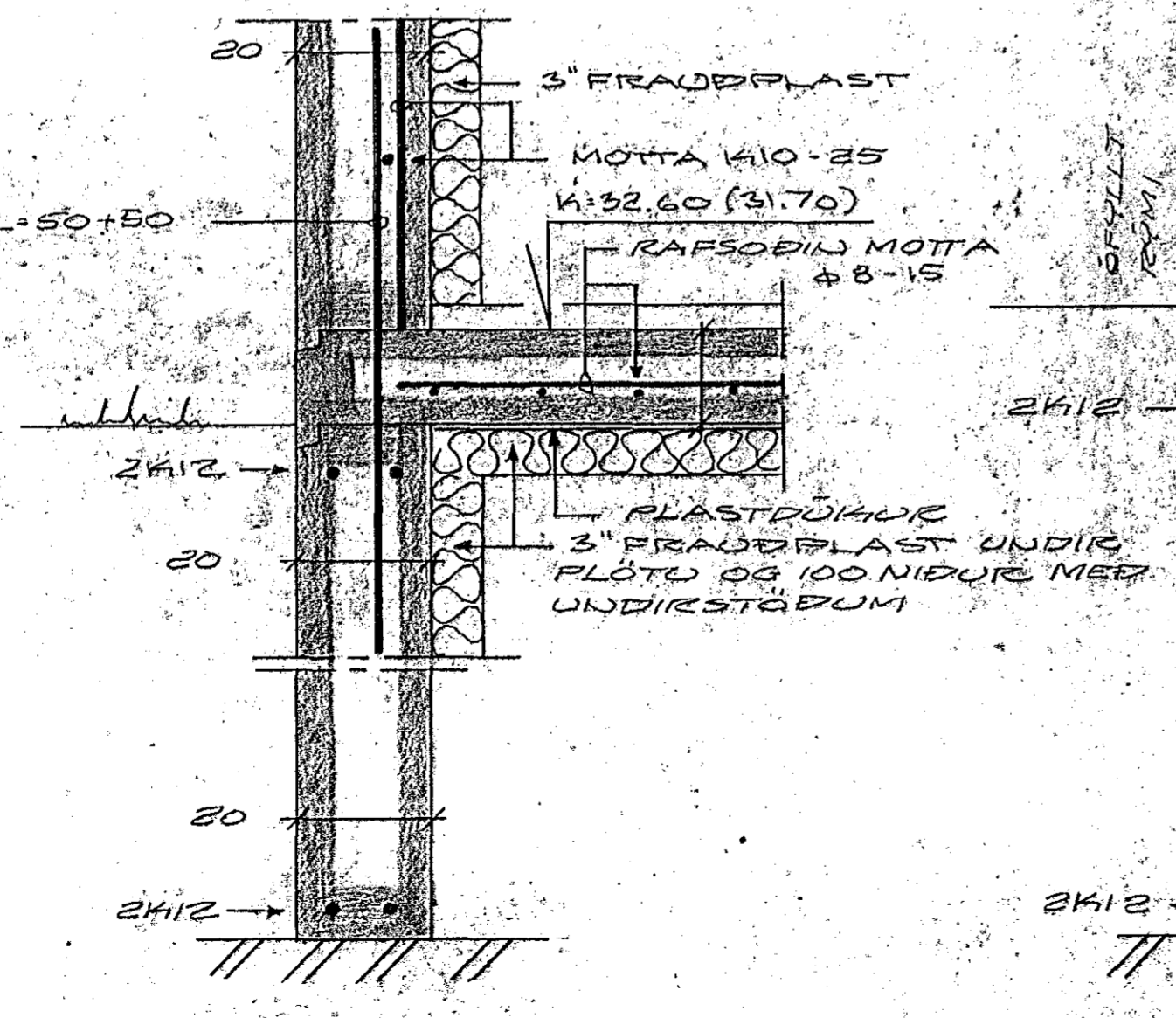
SNID B, M=1:10
