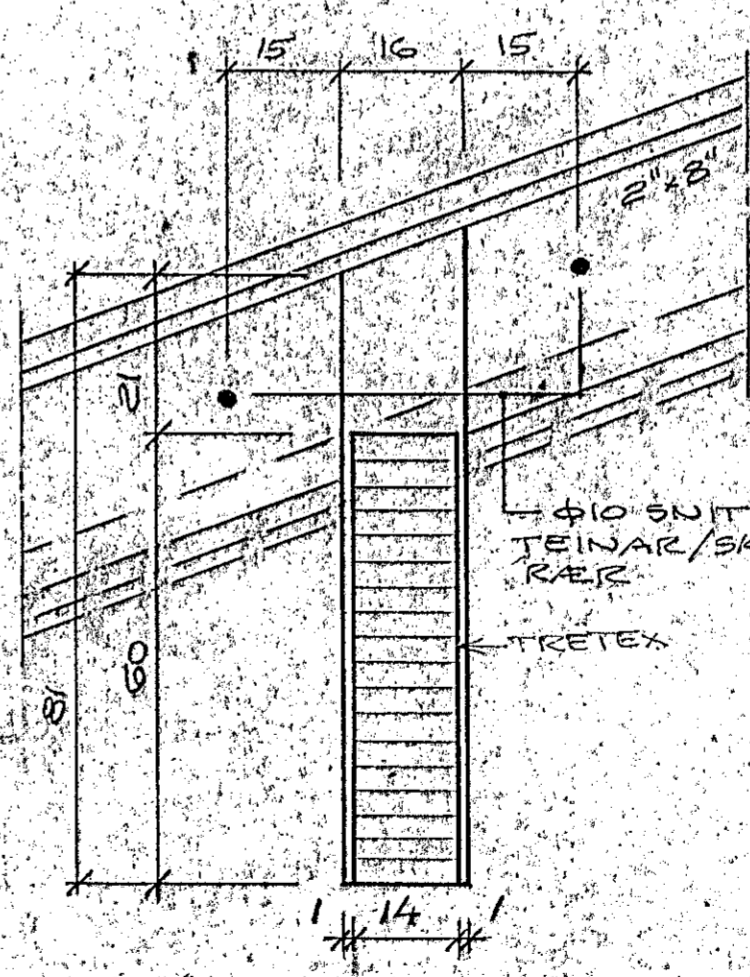
SNID P (P'), M=1:10 (SNID P' SPEGILVENDT)
