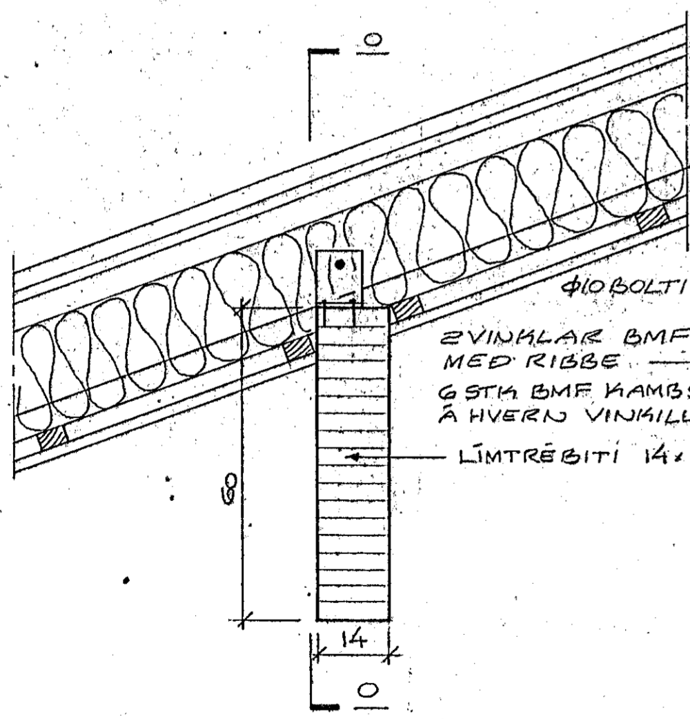
SNID L, M=1:10
