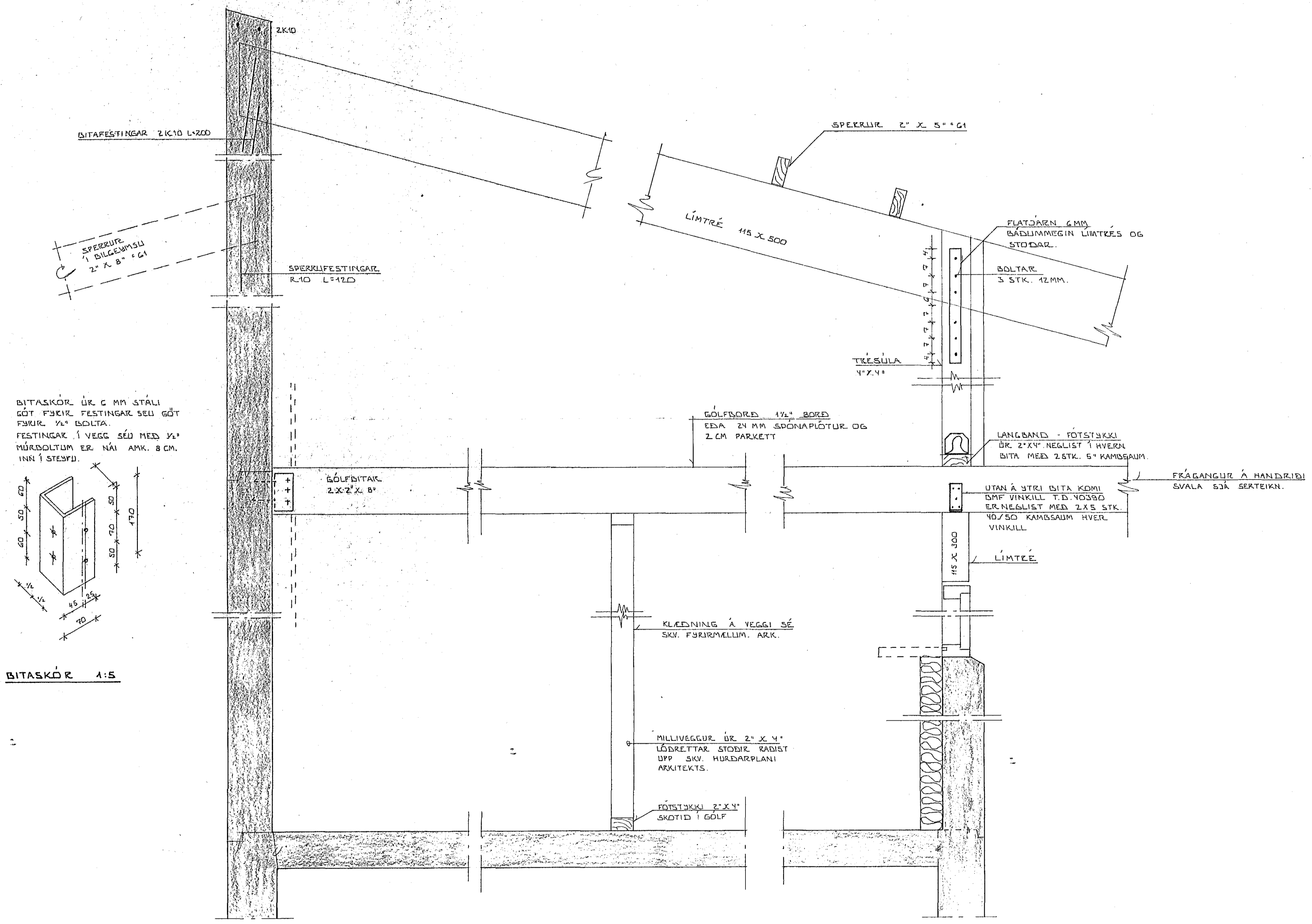
SNIED I HÚS 1:10
