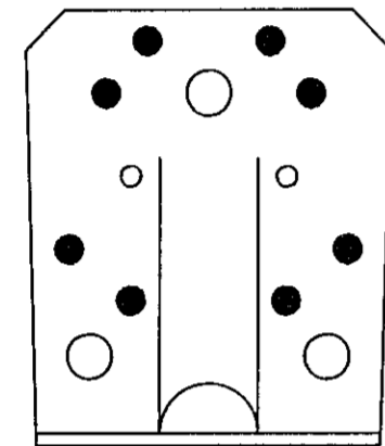
Negling 1 sperrur 8 stk BMF-kamsaumur 40/40
