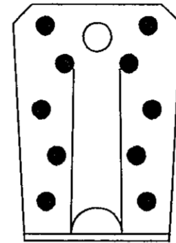
Negling 1 langbönd/stoðir 10 stk BMF-kamsaumur 40/40
