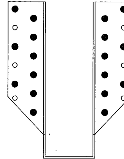
Negling 1 limtré 2*9 stk BMF-kamsaumur 40/50
