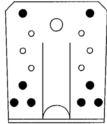
Negling 1 limtré 8 stk BMF-kamsaumur 40/60
