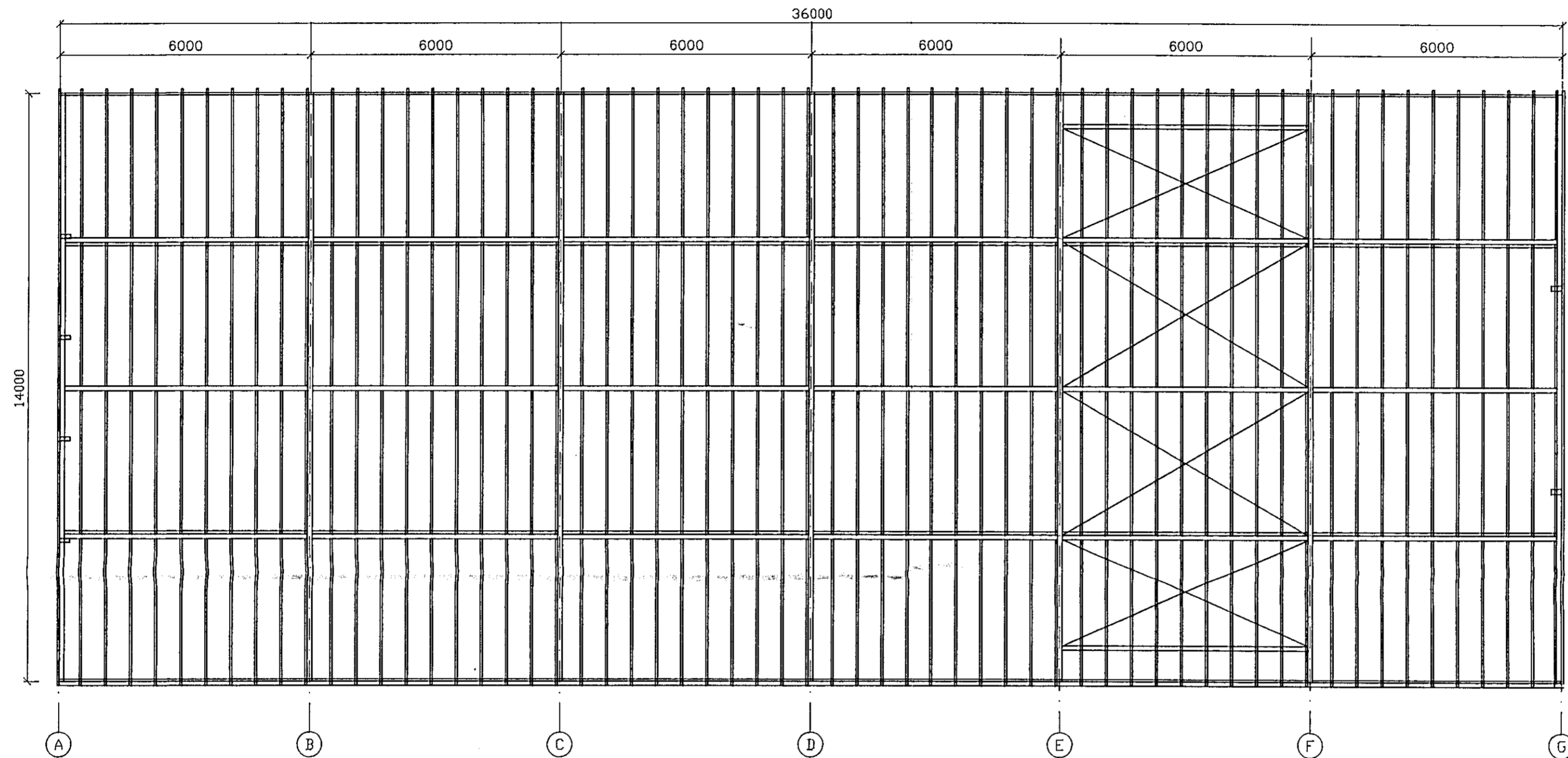
Þakplan Mkv. 1:100
