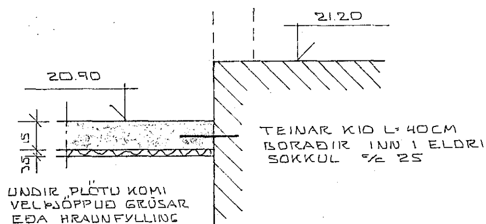
SNID B 1:20
