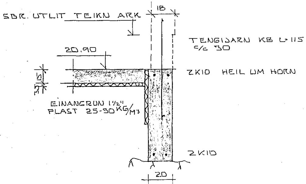
SNID A 1:20
