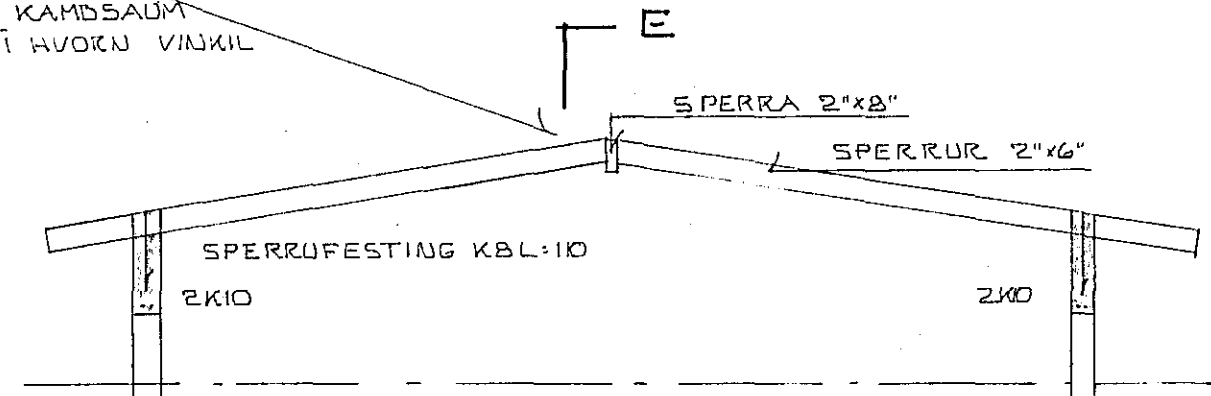
SNID C-C 1:50
