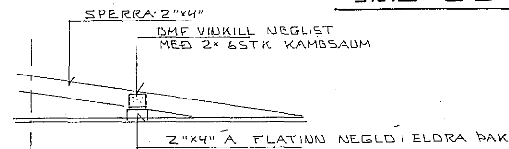
SNID F-F 1:20
