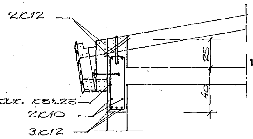
SNID A 1:20
