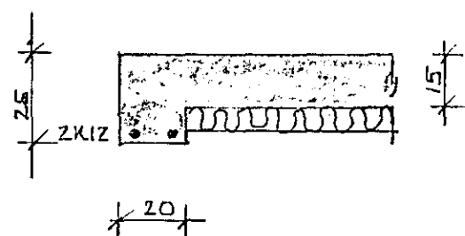
SNIB E-E 1:20
