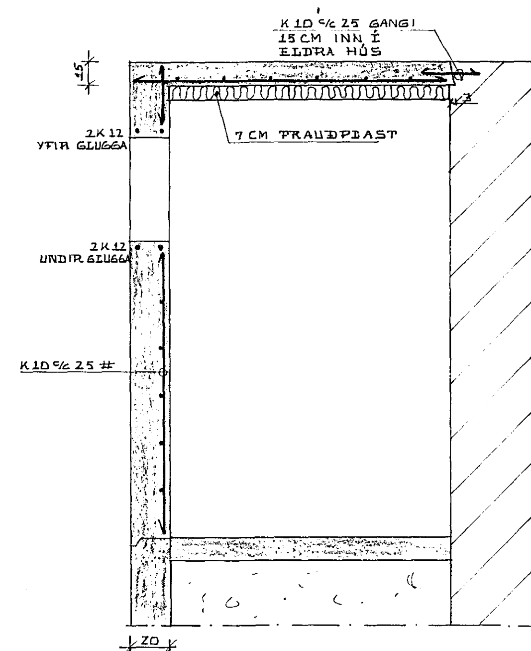
SNIB C-C 1:20
