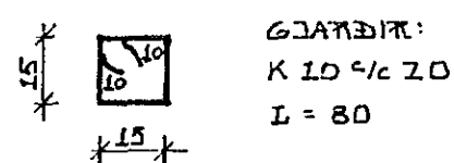
SNIB I SULU S1 1:20
