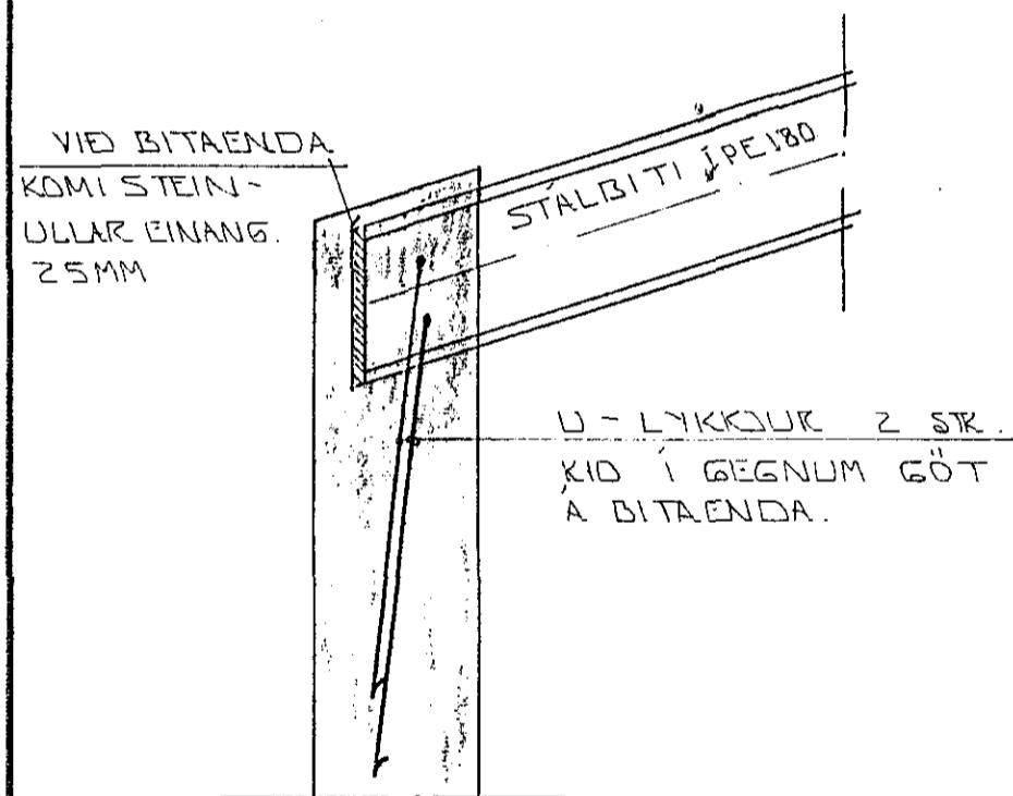
FRAGANGUR STALBITA I VEGG 1:10
