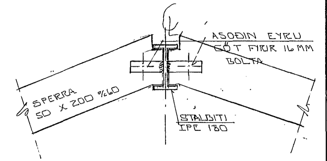
SNIED G - 1:10
