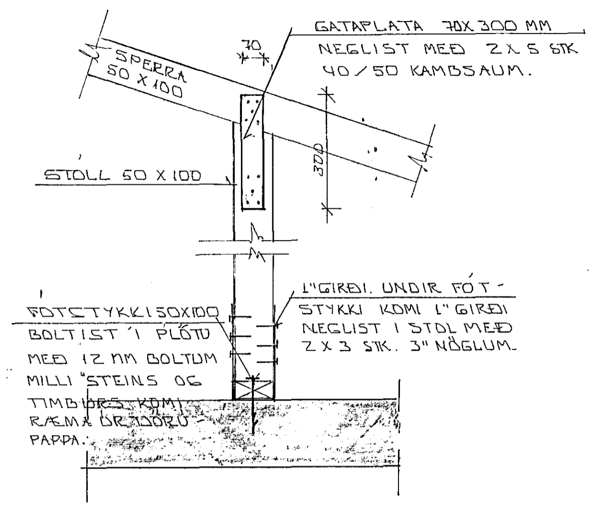
SNIED E - 1:10
