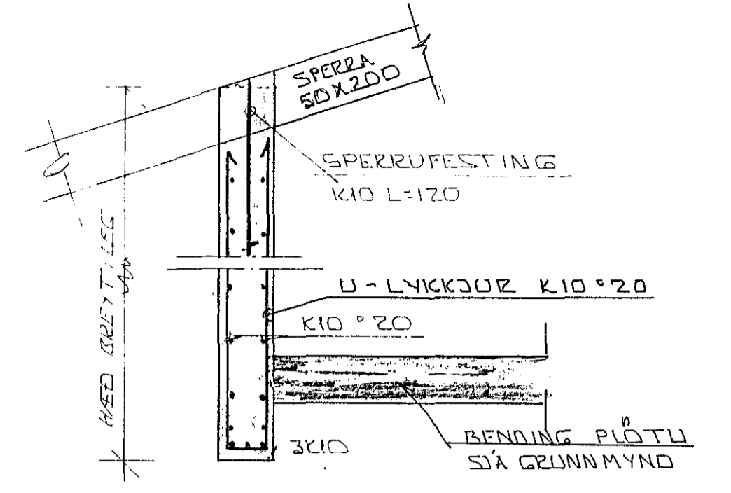
SNIED G YFIR BILG. DYRUM - 1:20
