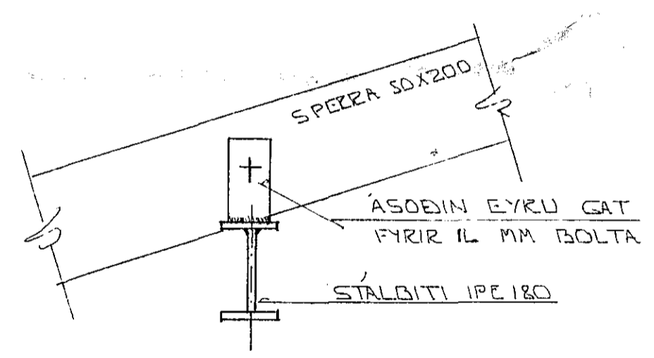
SNIED B - 1:10
