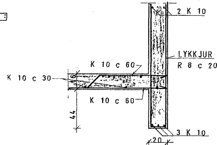
SNID A 1:20
