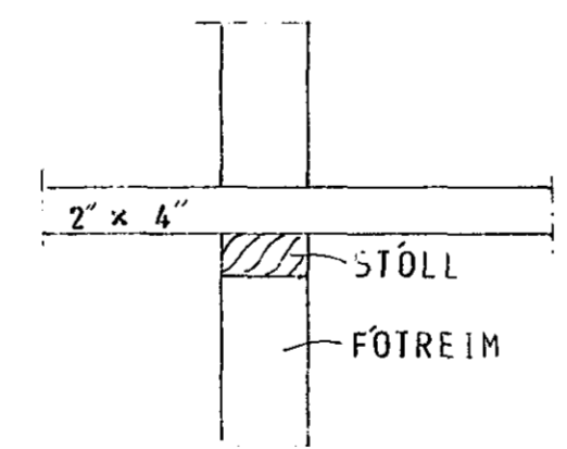
SNID A 2
