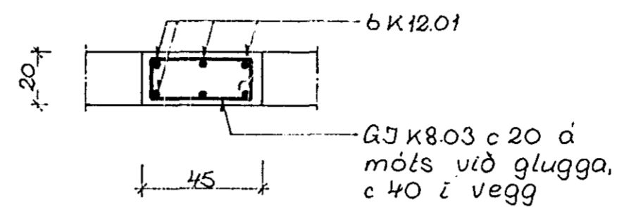
BITI B1.3. 2.stk. 1:20 B1.3' 1.stk.
