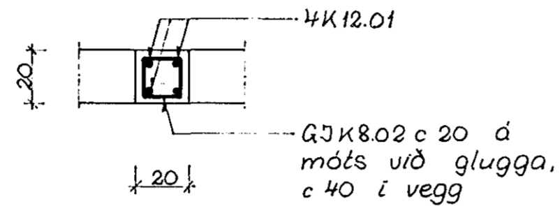
SNID X-X
