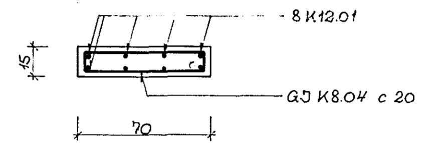
SNID Y-Y
