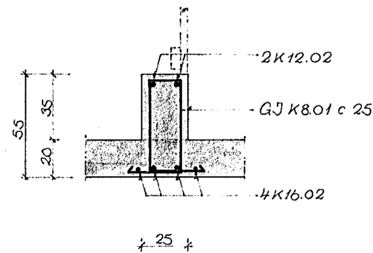
SNID B-B
