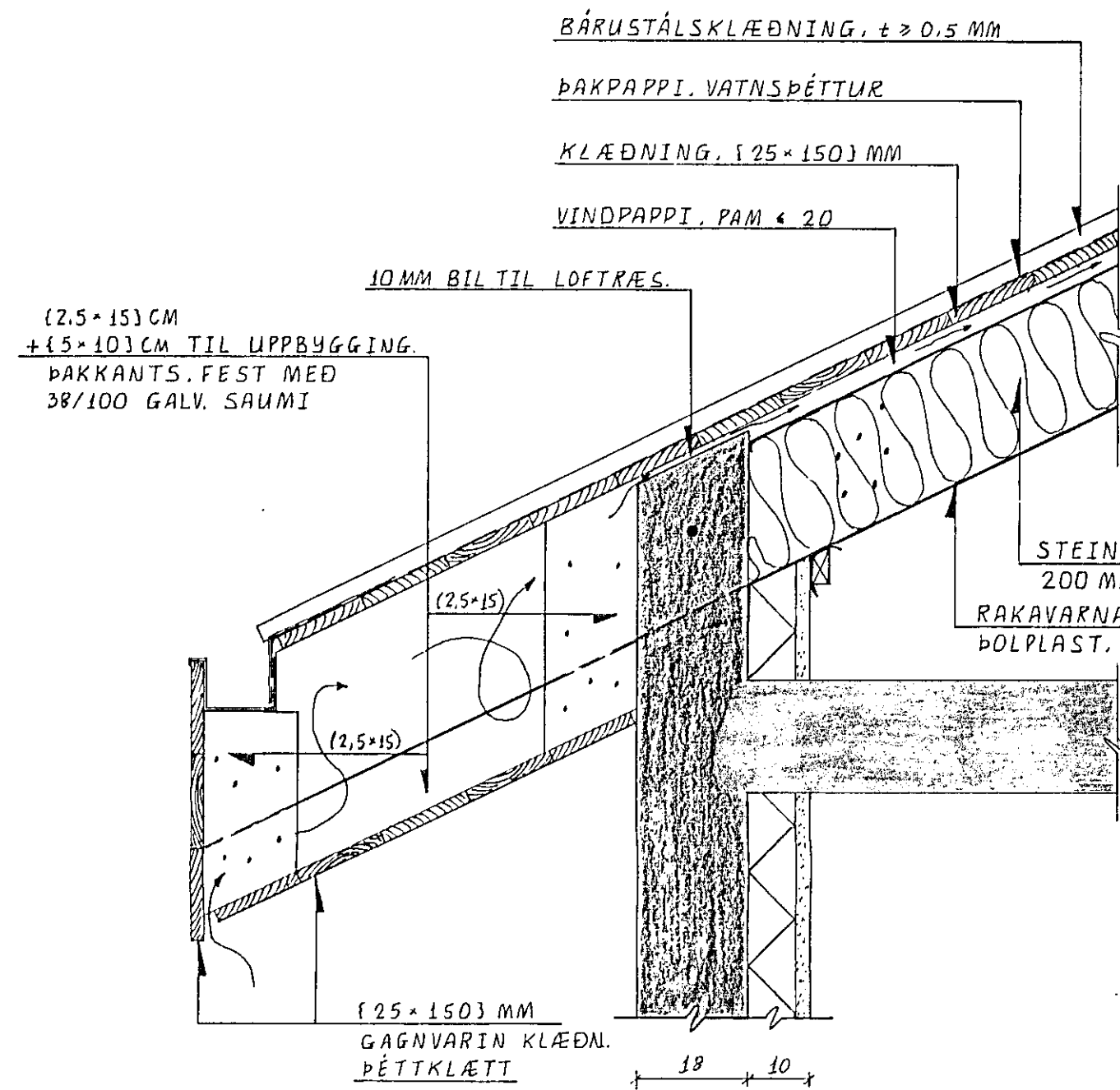
SNID A 12 -A 12 . 1:10
