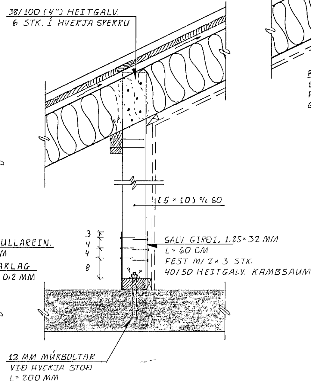
SNID B 12 -B 12 . 1:10
