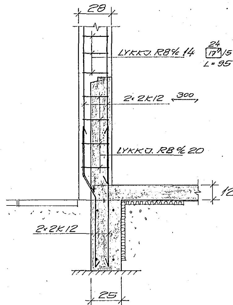
SNID "D-D" 1:20 BENDING I SÖLU S2
