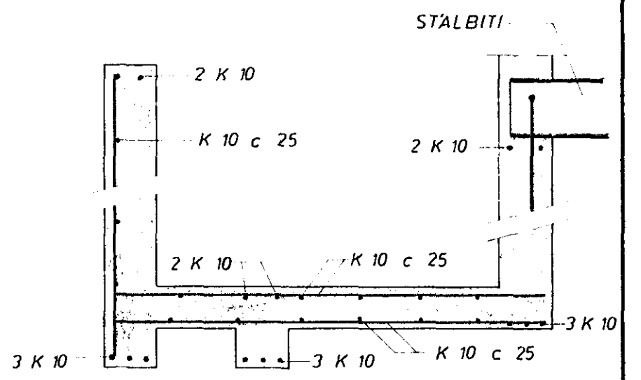
SNID C 1:20
