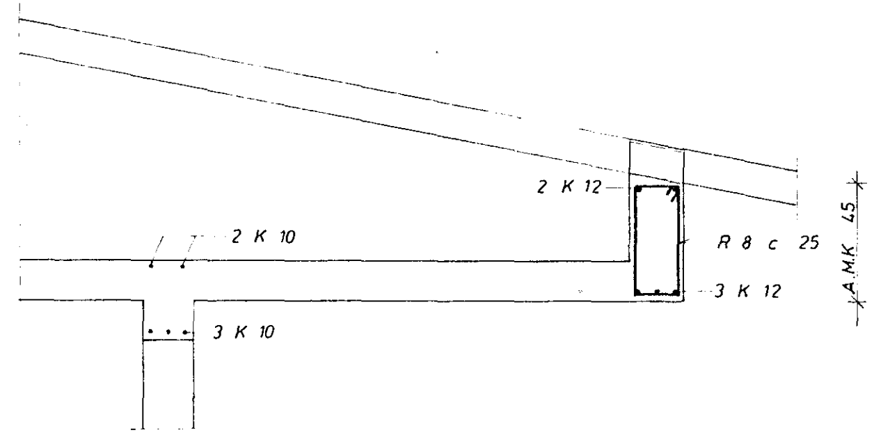
SNID A 1:20
