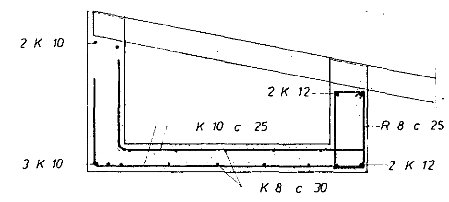
SNID B 1:20
