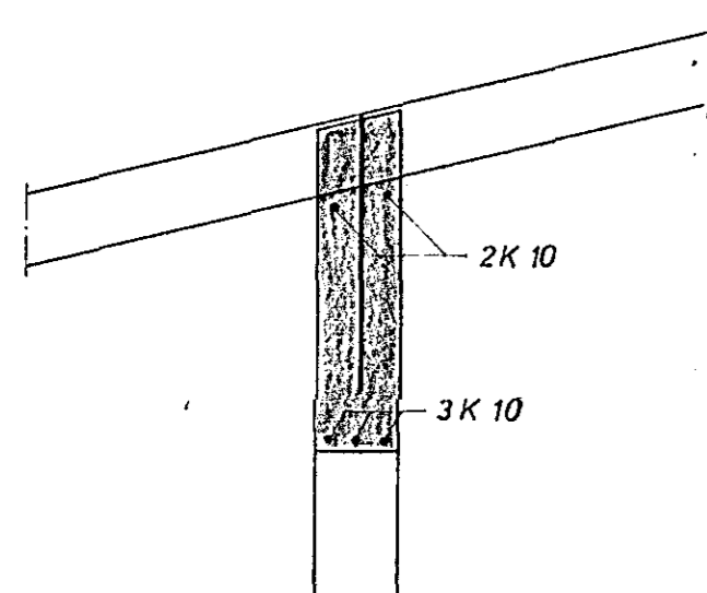
SNID F 1:20
