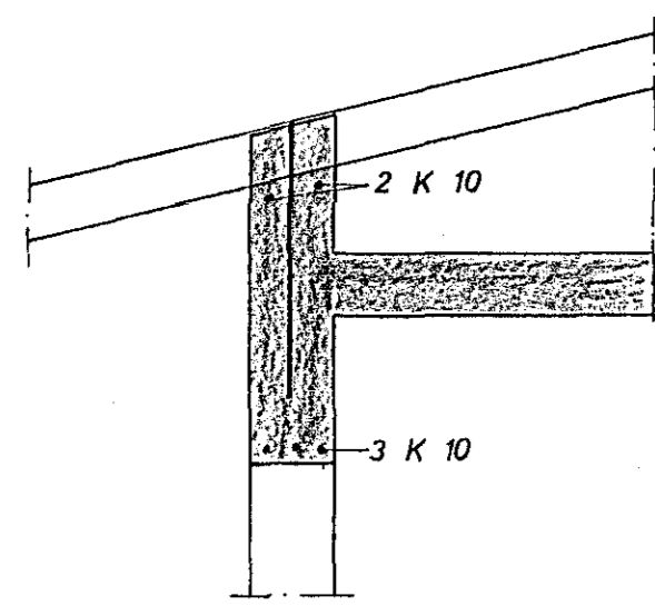
SNID A 1:20
