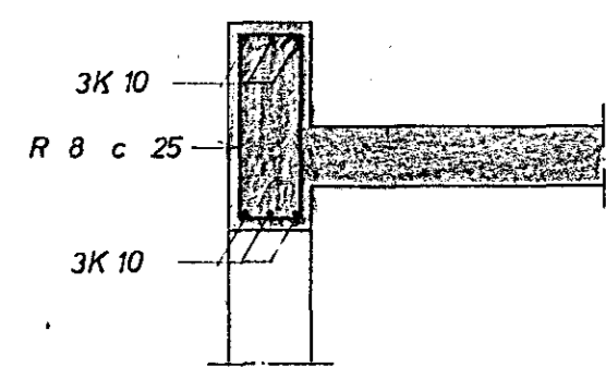
SNID C 1:20
