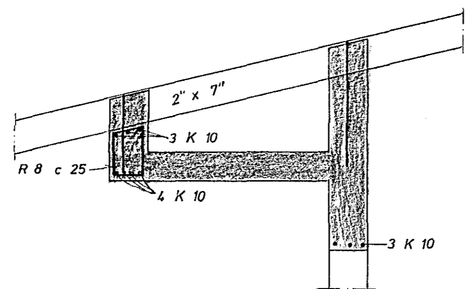
SNID B 1:20
