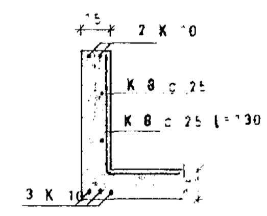
SNID C 1:20
