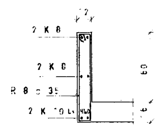
SNID A 1:20
