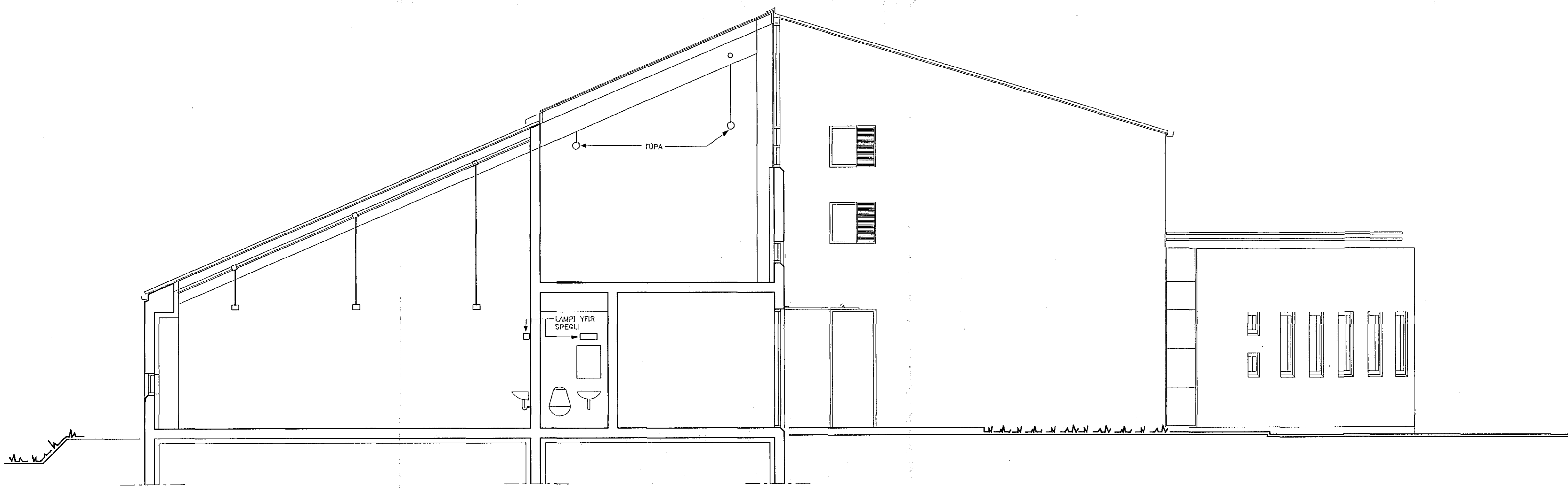
SNID B-B
