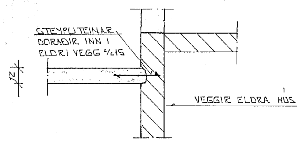
SNID 3 1:20
