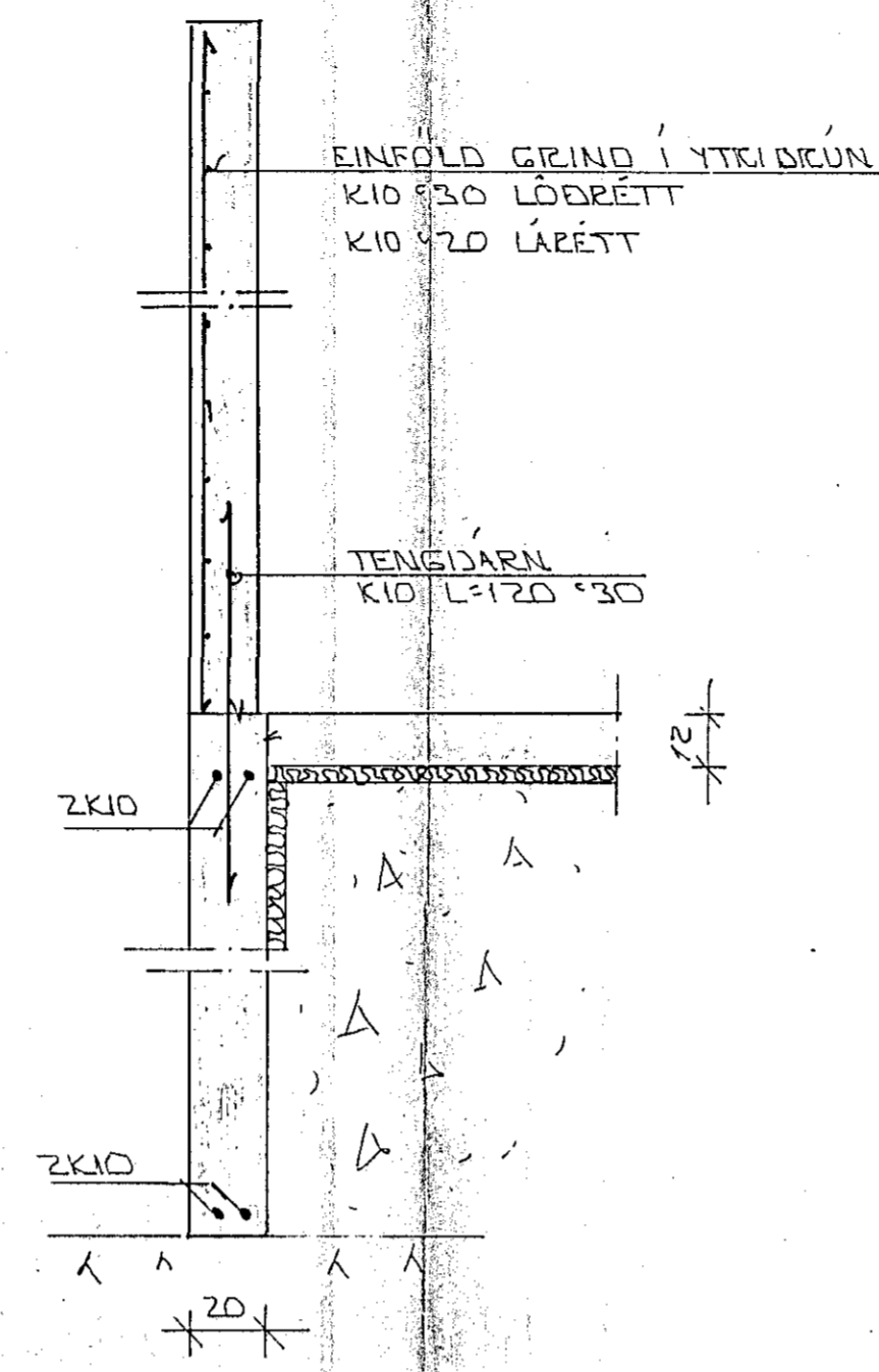
SNID 1 1:20
