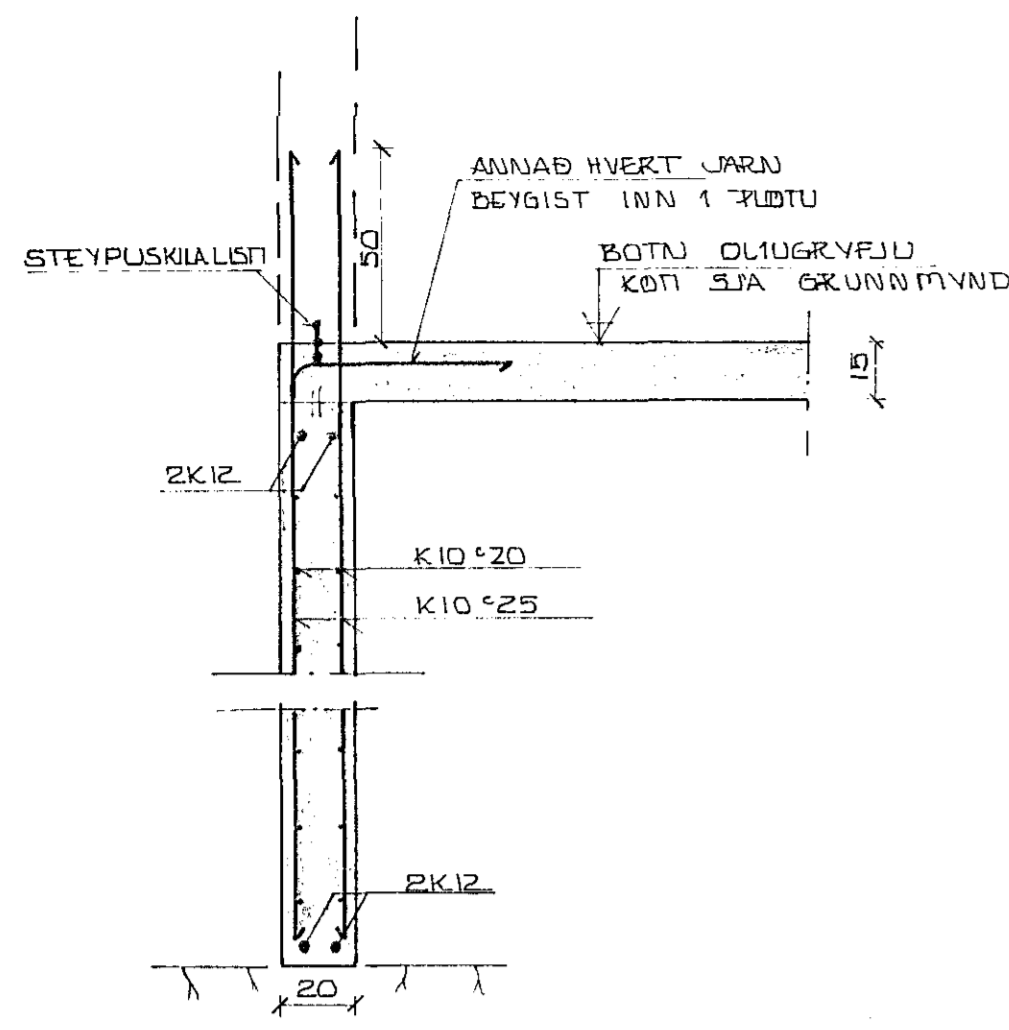
SNID A 1:20
