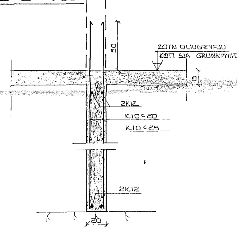
SNID N 1:20
