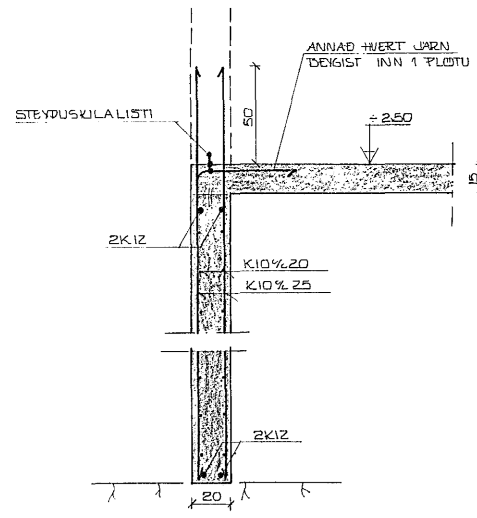
SNID B 1:20
