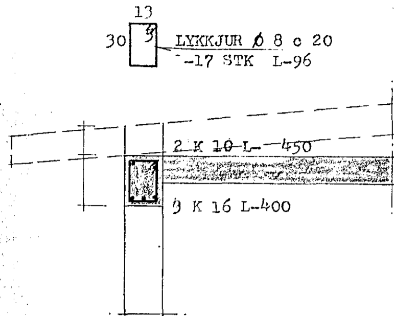
SNID - A 1:20
