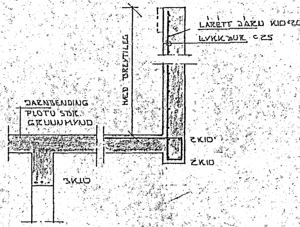
SNID B 1:20
