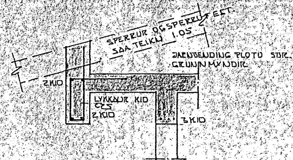
SNID A 1:20
