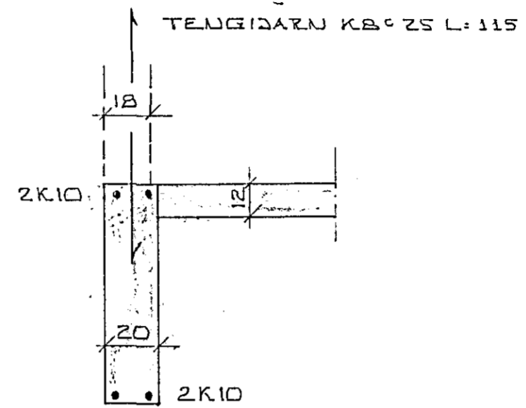
SNID A - A 1:20
