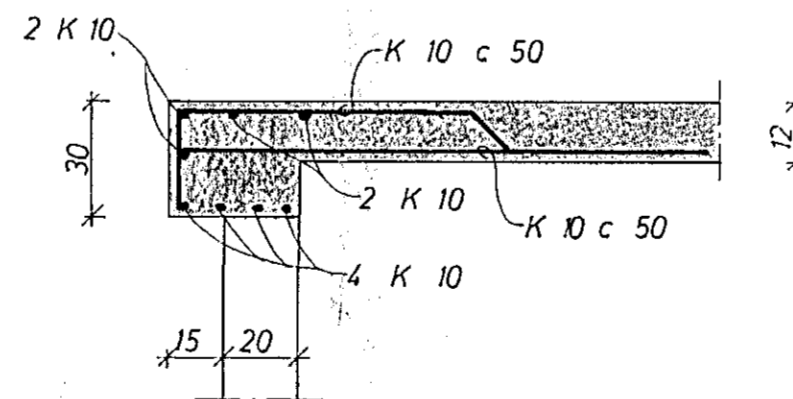
SNID A 1:20
