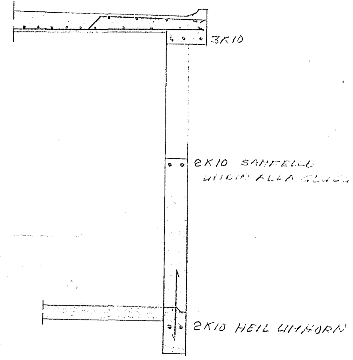
SNID I GLUGGAHLIDAR - 1:20 -
