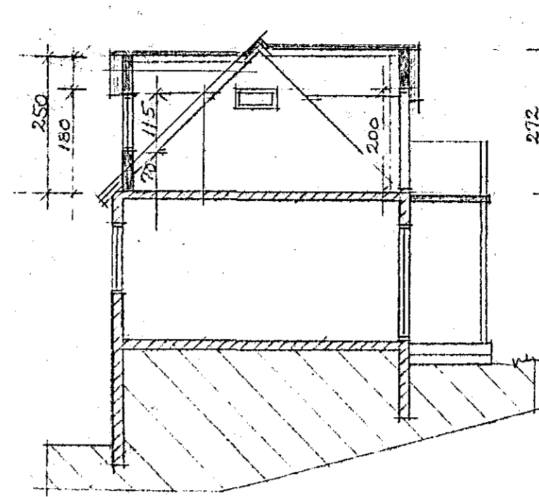
SNIP 1:100
