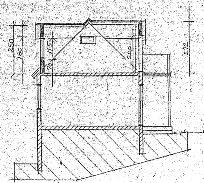
SNIP 1:100
