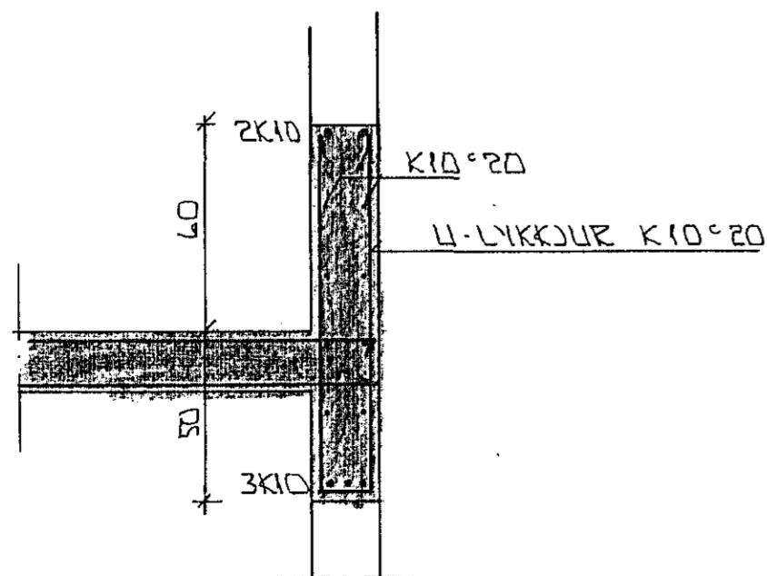
SNID 6 x 1:20
