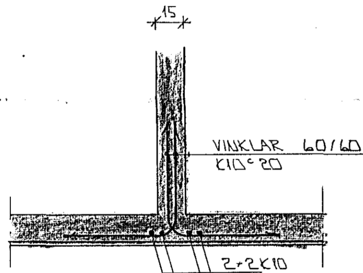
SNID 5 x 1:20
