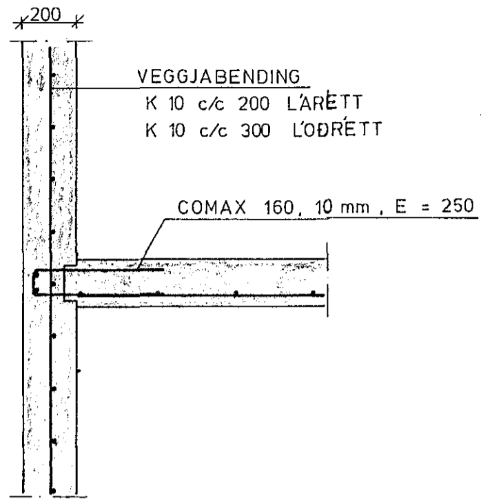
SNID B 1:20
