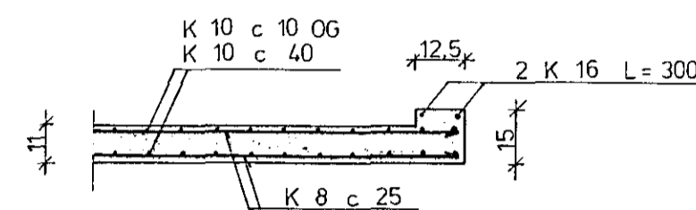
SNID B 1:20
