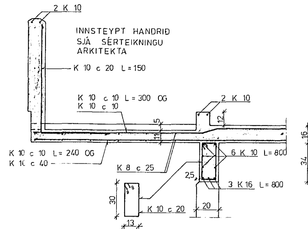
SNID A 1:20
