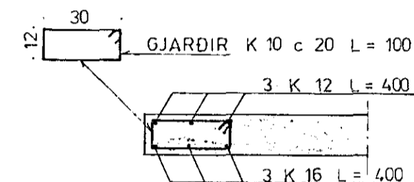
SNID C 1:20
