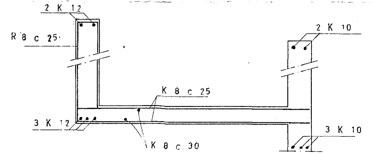
SNID C 1:20
