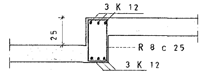
SNID A 1:20
