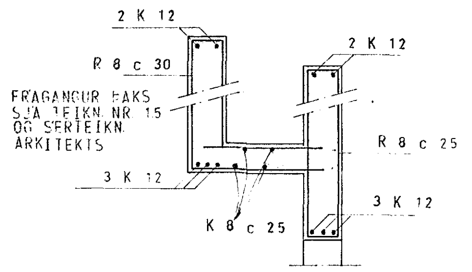
SNID B 1:20
