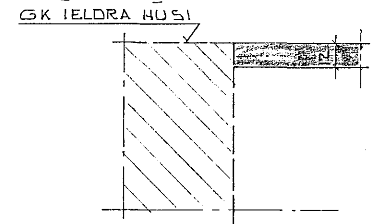
SNID B 1:20
