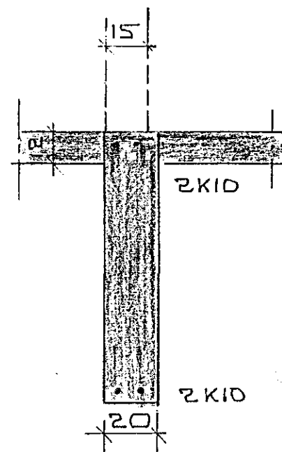
SNID C 1:20
