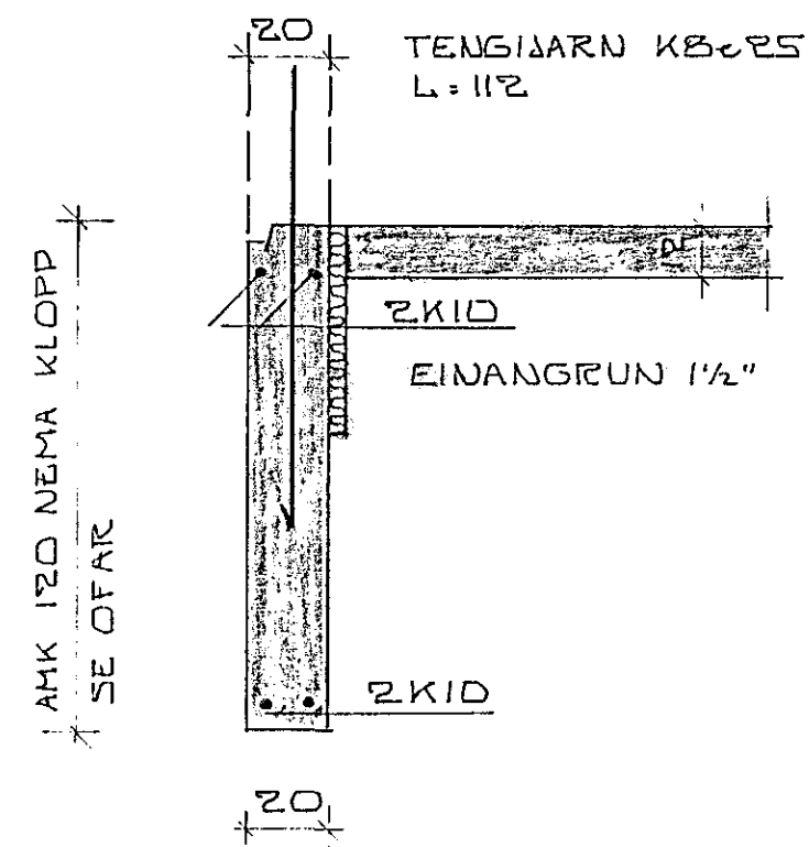
SNID A 1:20
