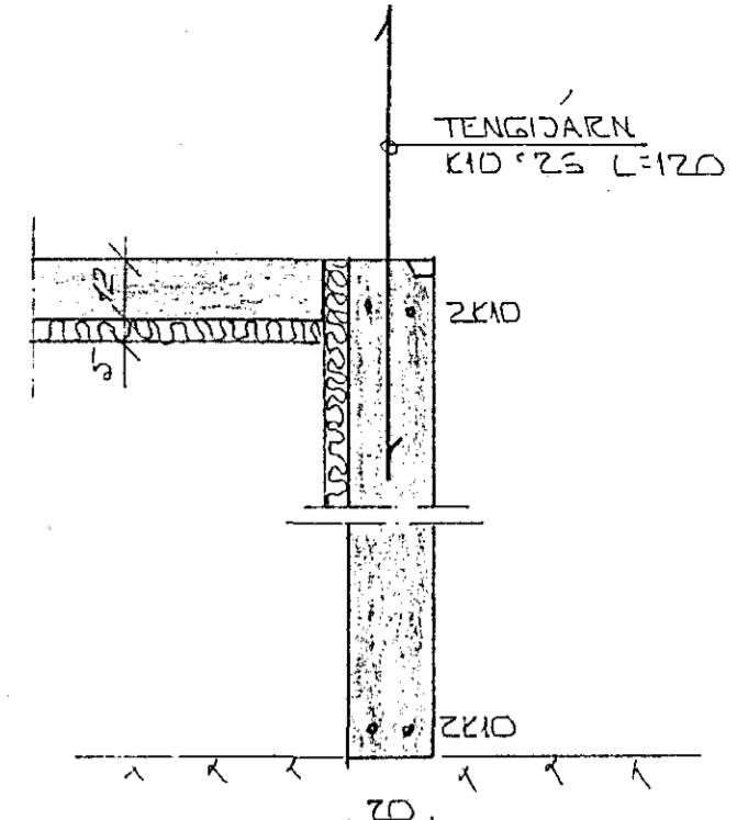
SNID 1 1:20
