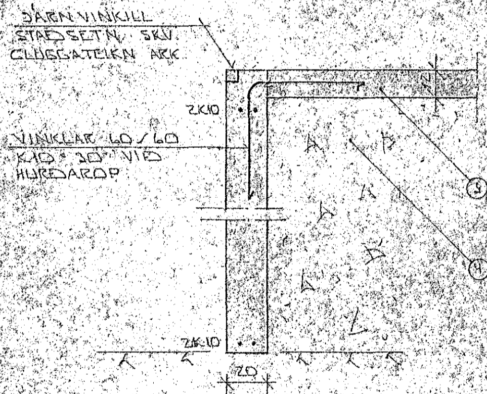
SNID 2 I HURDAROP A BILG. 1:20
