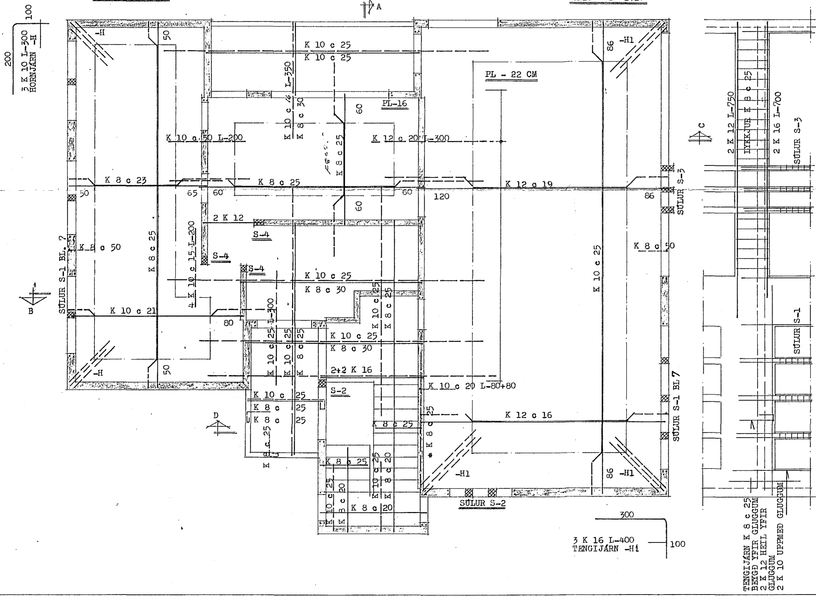
SNID - A 1:20
