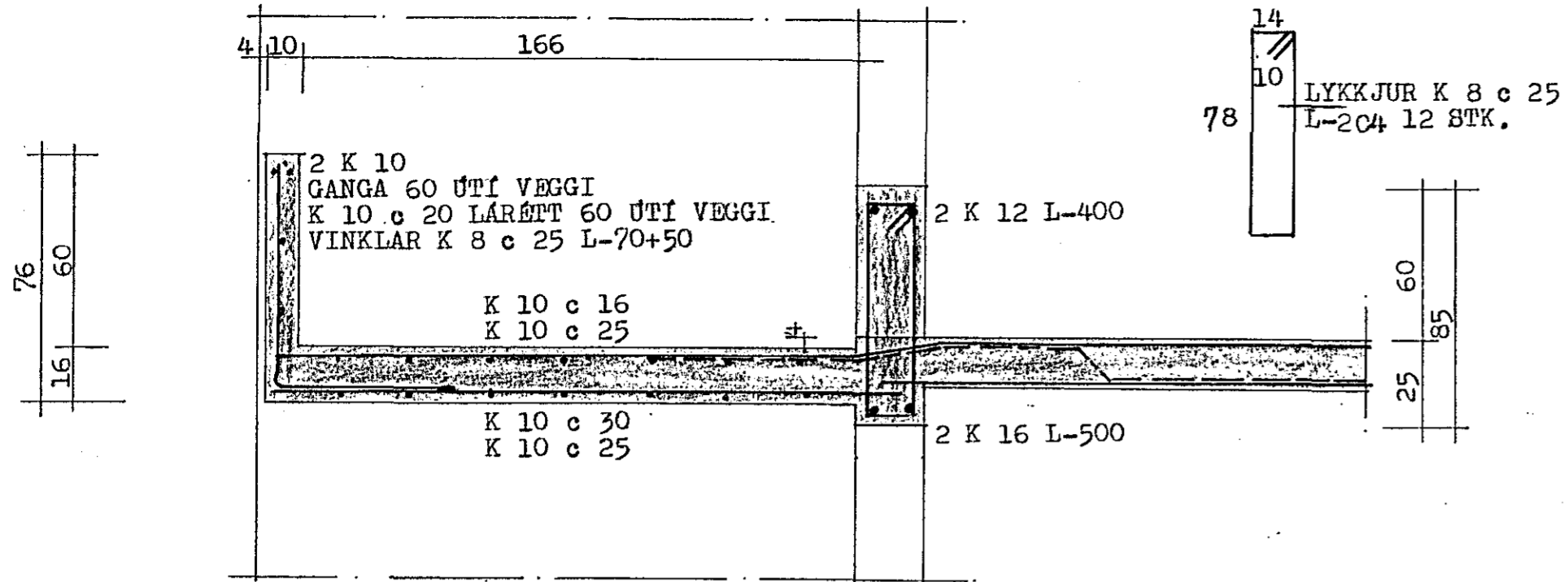
SNID - A 1:20
