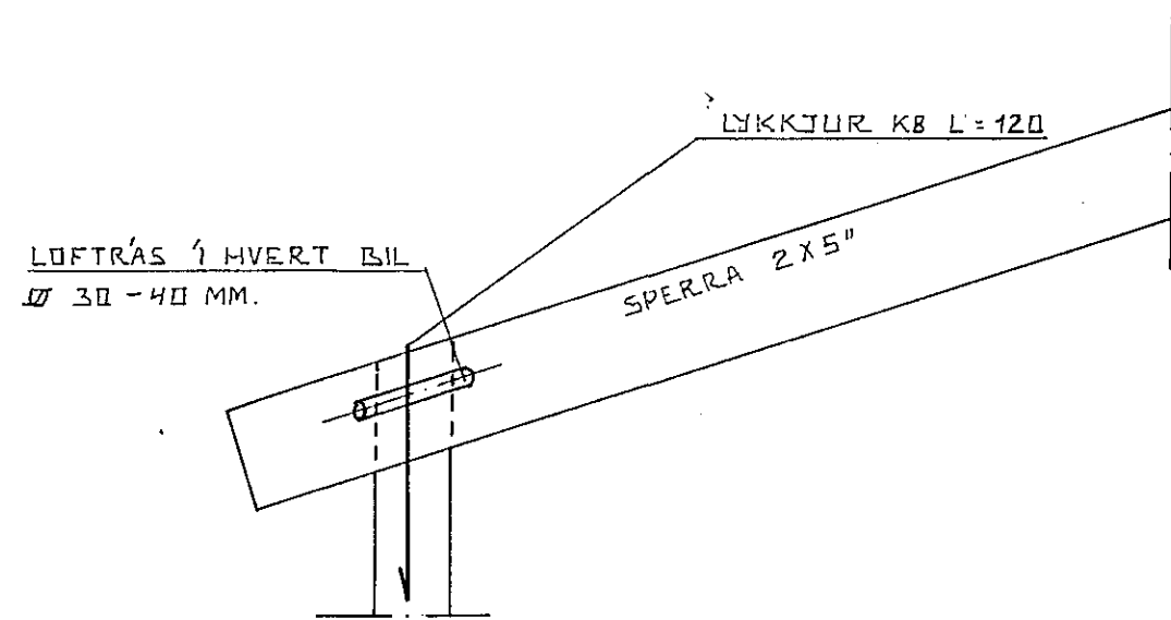
SNID C-C 1:10
