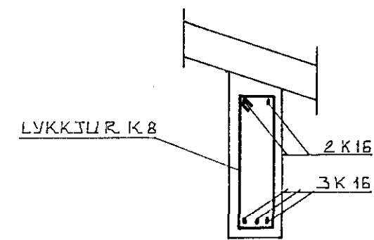
SNID E-E 1:20
