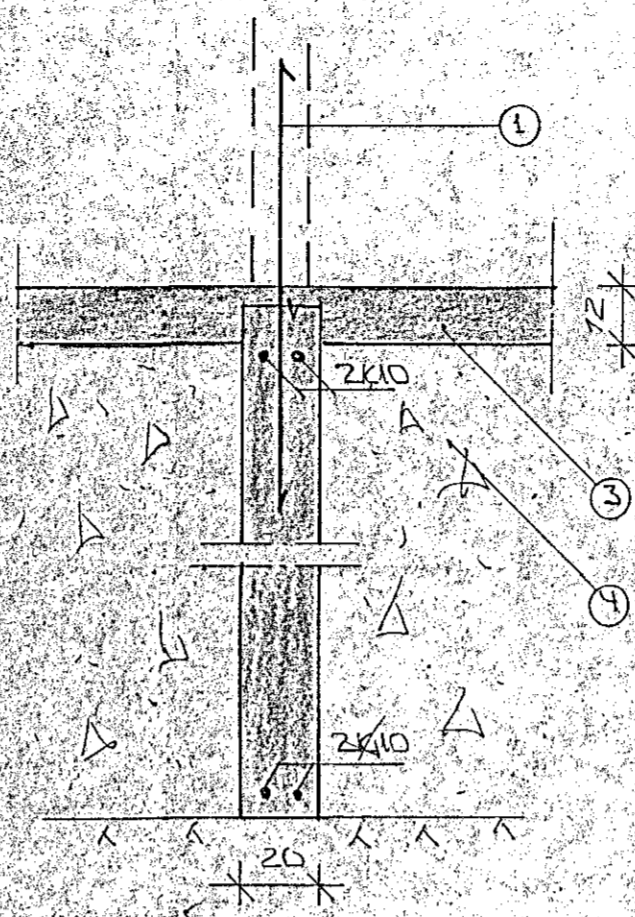
SNID 3 1:20
