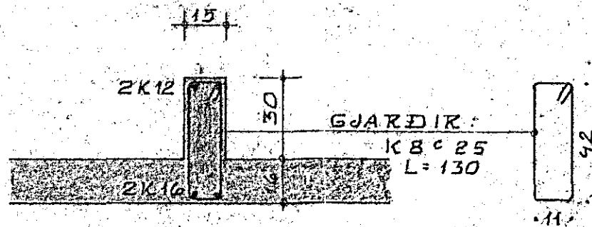
SNID 2-2 1:20
