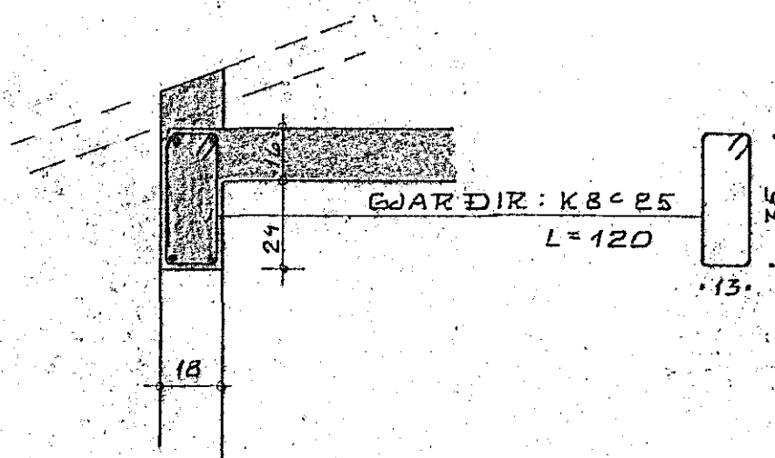
SNID 5-5 1:20
