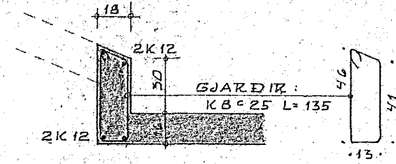
SNID 3-3 1:20
