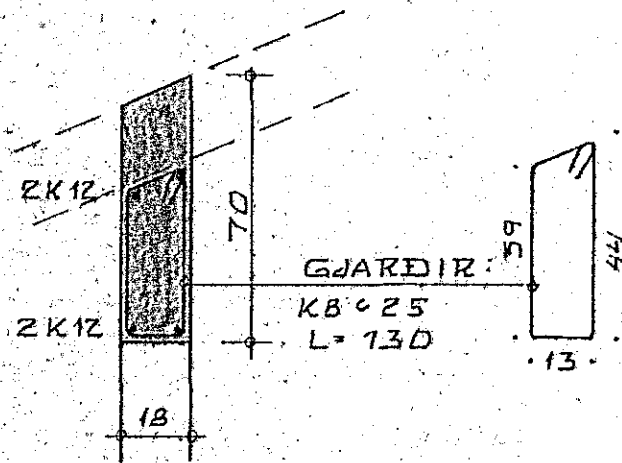
SNID 4-4 1:20
