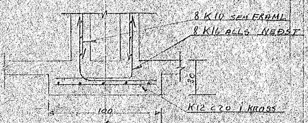
SNID I SKORSTEIN 1:20
