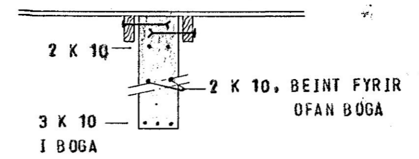
SNID B 1:20
