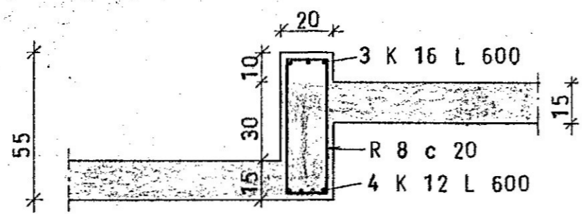
SNID F 1:20
