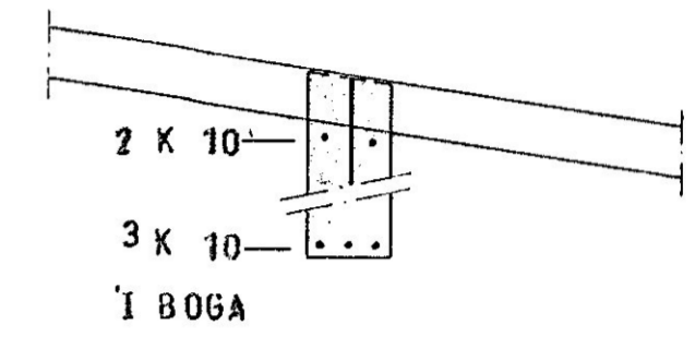
SNID C 1:20
