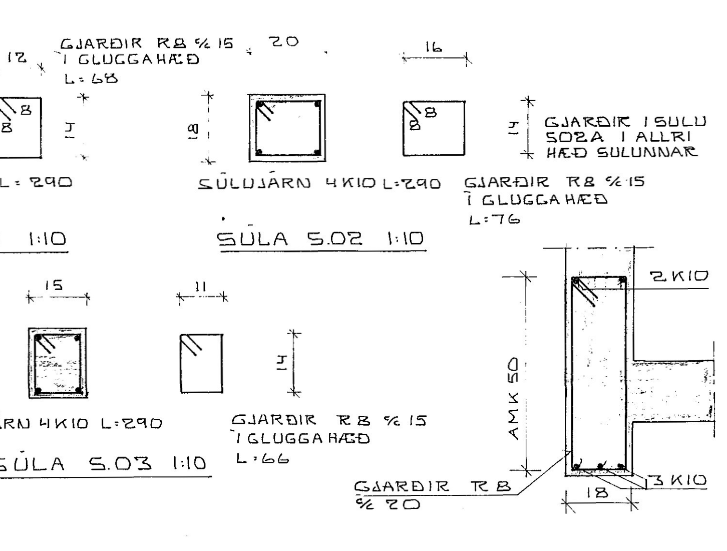
SNIDA-A 1:10
