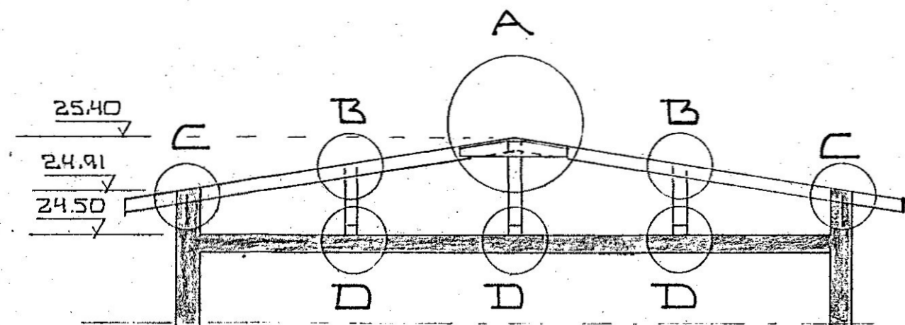
SNID C-C 1:50
