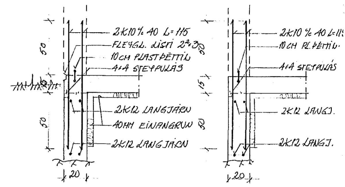
SNID C, 1:20
