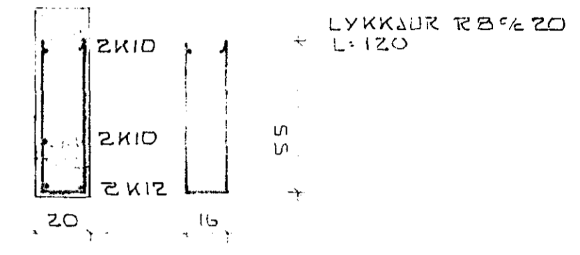
SNID C-C 1:20
