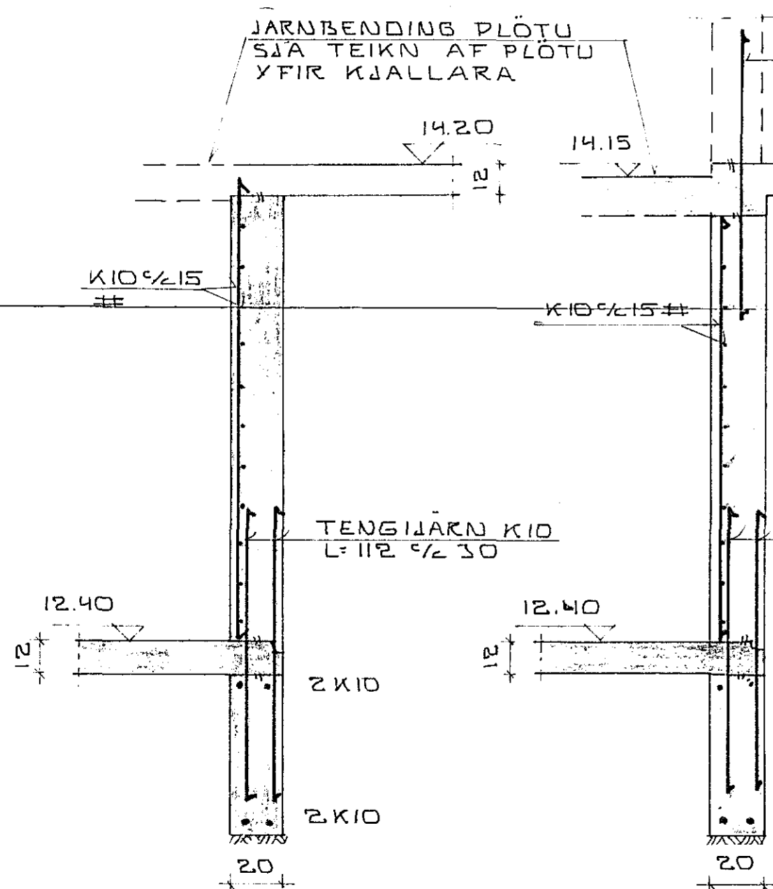
SNID J-J
