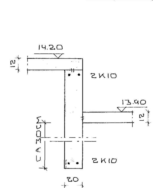
SNID F-F
