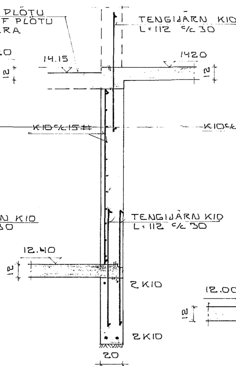
SNID J-J
