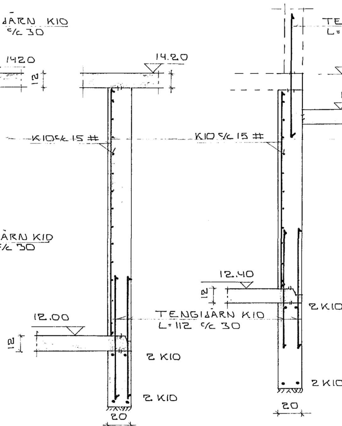
SNID L-L
