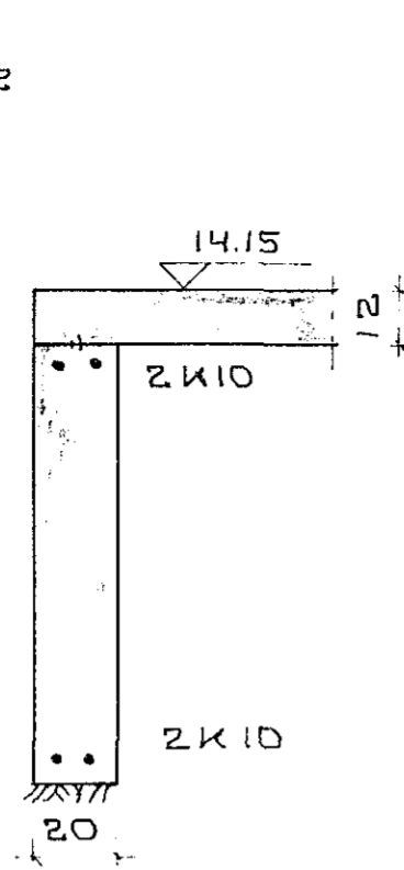
SNID B-B
