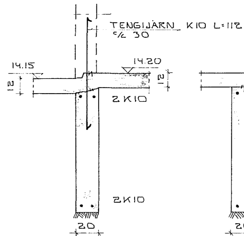
SNID C-C
